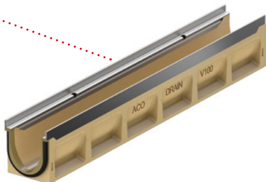
Multiline Seal in Zarge: Edelstahl
