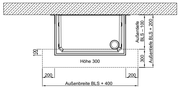
Fundament Option 2
